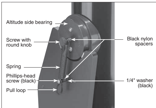
Figure 6. Close-up view of the CorrectTension system, which pulls the tube assembly down onto the altitude bearing pads.
