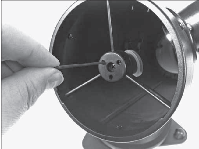
Figure 6. Adjust the tilt of the secondary mirror with the three recessed setscrews surrounding the center screw.
