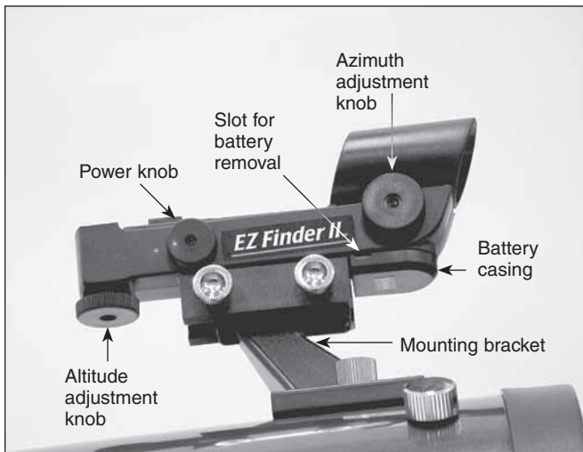
Figure 4. The EZ Finder II's On/Off and adjustment knobs.
