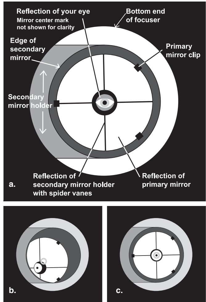
Figure 5. Collimating the optics. (a) When the mirrors are properly aligned, the view down the focuser drawtube should look like this. (b) Here, the secondary mirror is centered under the focuser, but it needs to be adjusted (tilted) so that the entire primary mirror is visible. (c) When the mirror is correctly aligned, the center "dot" of the collimation cap will be centered.
