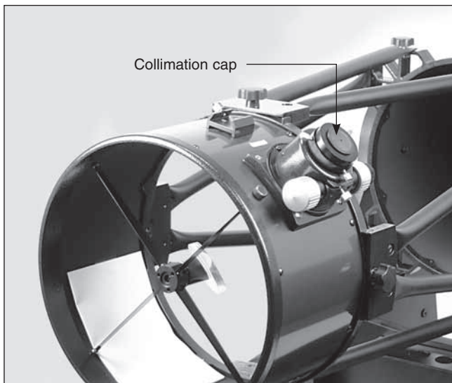
Figure 29. The SkyQuest optical tube properly set up for collimation.
