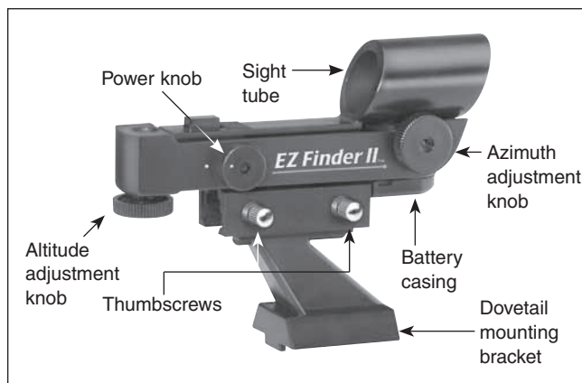
Figure 26. The EZ Finder II reflex sight.
