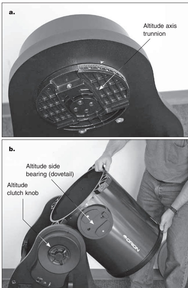
Figure 18. a) Altitude axis trunnion on left side panel. b) Grasp both ends of the lower tube section to lift it, then lower it into the base, sliding the dovetail slot in the tube's left altitude bearing into the mating part of the trunnion.
