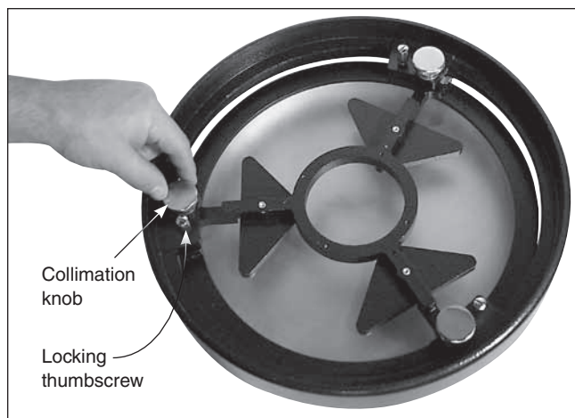
Figure 32. The tilt of the primary mirror is adjusted by turning one or more of the three larger thumbscrews. (XX12g shown)
