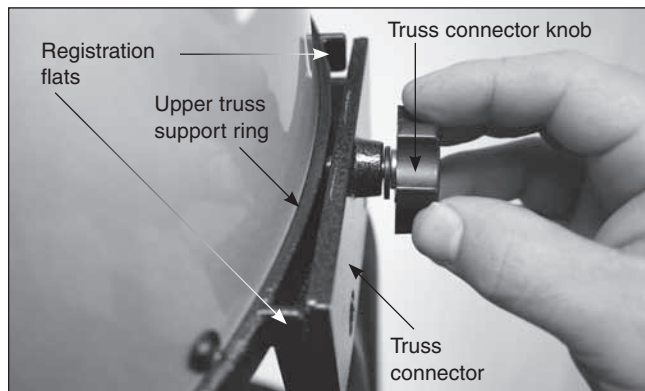
Figure 24. When the truss clamping knob is tightened, it will clamp the truss connector against the registration flats on the upper truss support ring.
