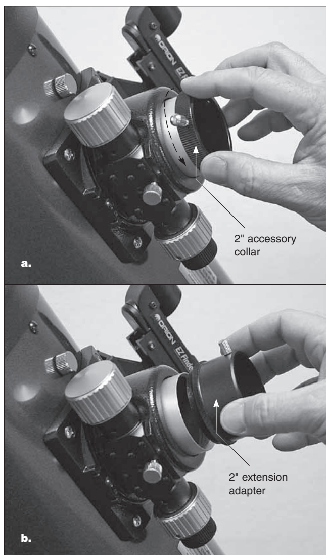
Figure 35. (a) Removing the 2" accessory collar, (b) Thread the 2" extension adapter into the focuser drawtube.
