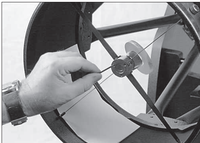
Figure 31. Adjust the tilt of the secondary mirror by adjusting one or more of the three alignment setscrews with a 2mm hex key.
