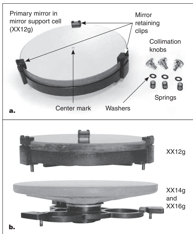
Figure 3. Contents of the primary mirror box. a) The primary mirror, mirror cell, and collimation hardware for the XX12g. b) The primary mirrors and mirror support cells for the XX12g (top) and XX14g/XX16g are quite different.
