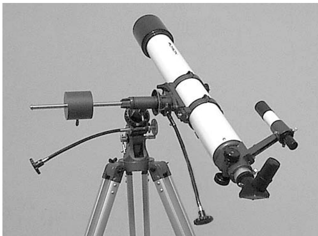
Figure 6a. Telescope pointing south. Note that in all these illustrations, the mount and tripod remain stationary; only the R.A. and Dec. axes are moved.
