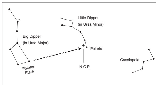
Figure 5. To find Polaris in the night sky, look north and find the Big Dipper. Extend an imaginary line from the two “Pointer Stars” in the bowl of the Big Dipper. Go about five times the distance between those stars and you'll reach Polaris, which lies within 1° of the north celestial pole (NCP).
