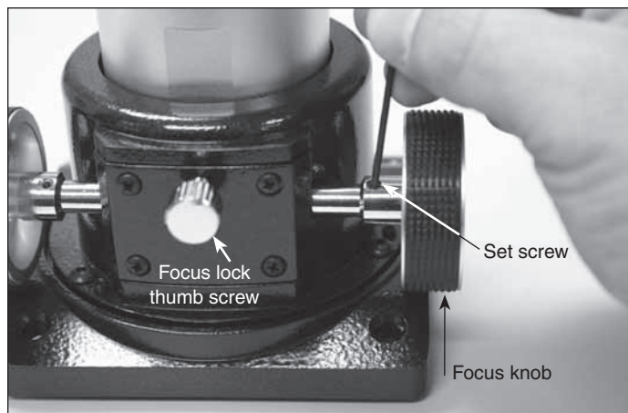
Figure 2. To remove the focus knob from the focusing shaft, first loosen the set screw on the knob’s stem.
