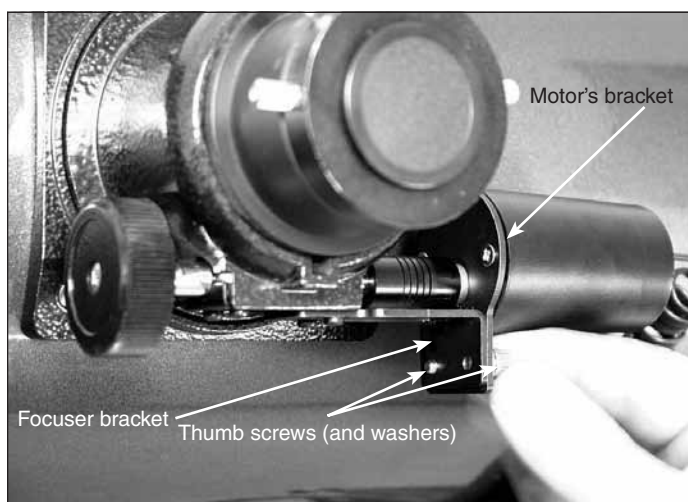
Figure 10. Connect the motor's bracket to the focuser bracket with the two thumb screws (and washers). The brackets should be flush against each other.
