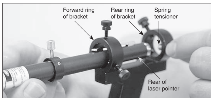
Figure 3. To insert the laser into the bracket, the rear of the laser pointer should first pass through the forward ring of the bracket. To pass the laser through the rear ring, you must pull the spring tensioner with your fingers.
